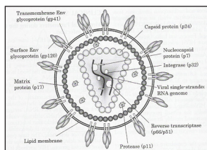
Schematic representation of a mature HIV virion showing the localization of viral proteins.
